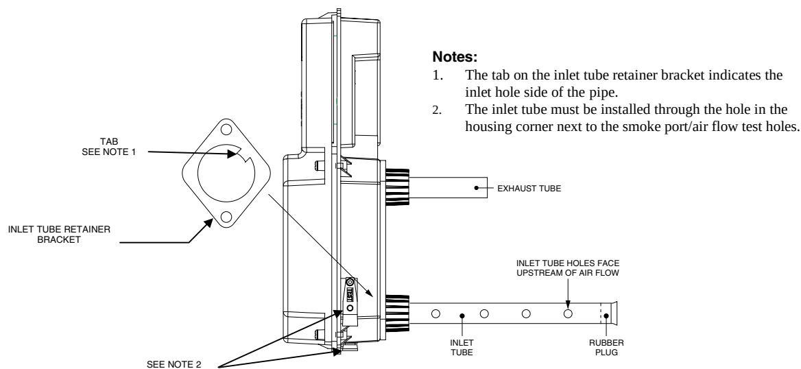
Figure 14. Inlet Tube Installation
