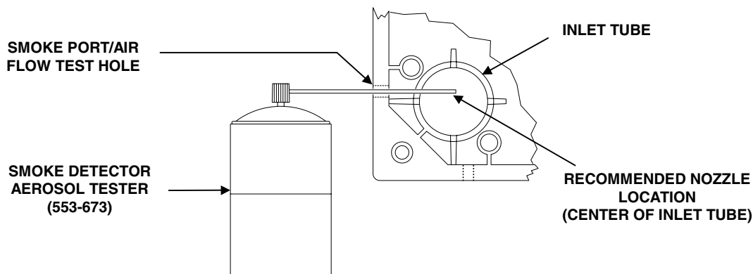
Figure 17. Smoke Detector Aerosol Test
