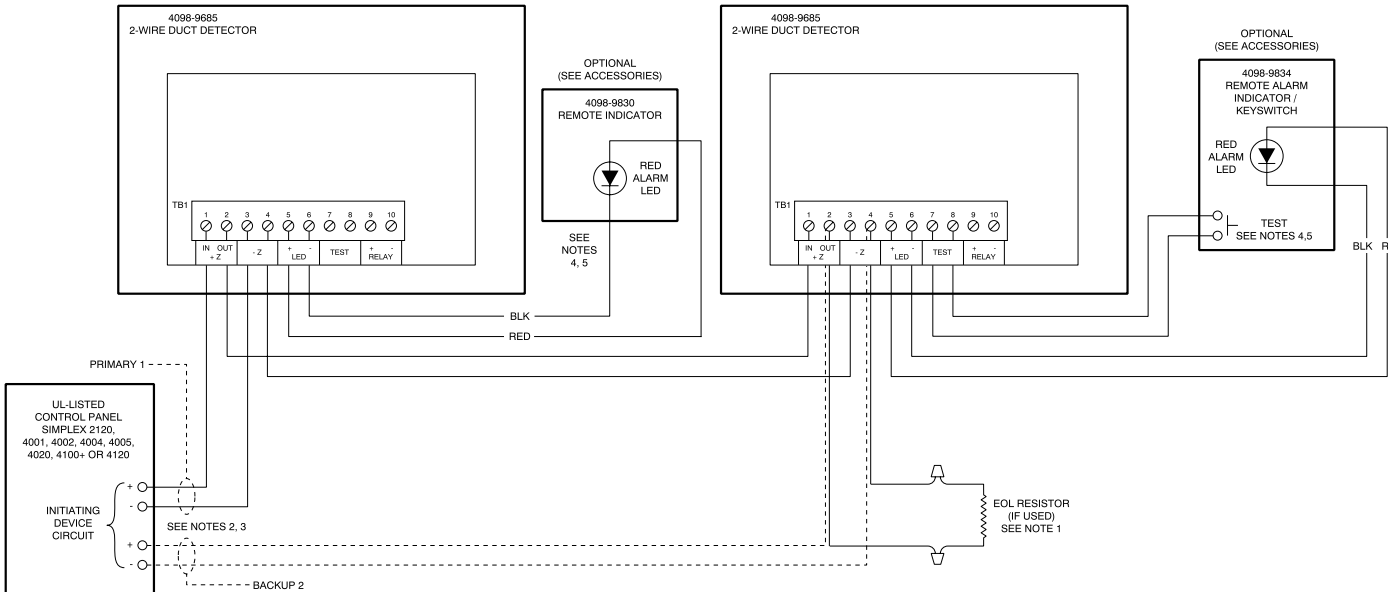
Figure 6. 4098-9685 Two-Wire Duct Detector DC Operation
