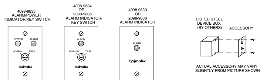
Figure 15. Accessory Installation
