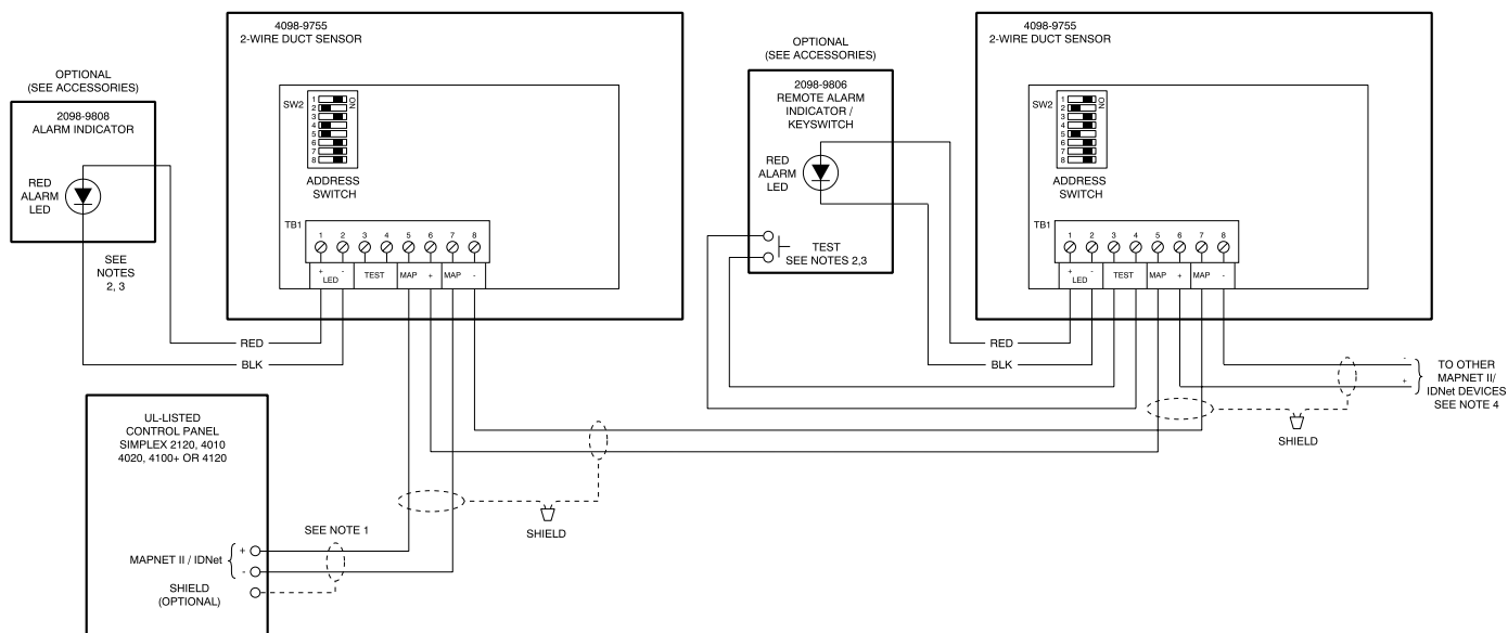
Figure 4. 4098-9755 Two-Wire Duct Sensor MAPNET II/IDNet Operation
