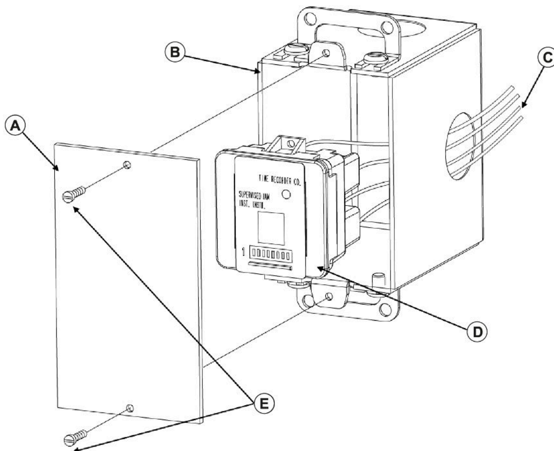
Figure 3: Mounting reference, single gang blank cover plate
