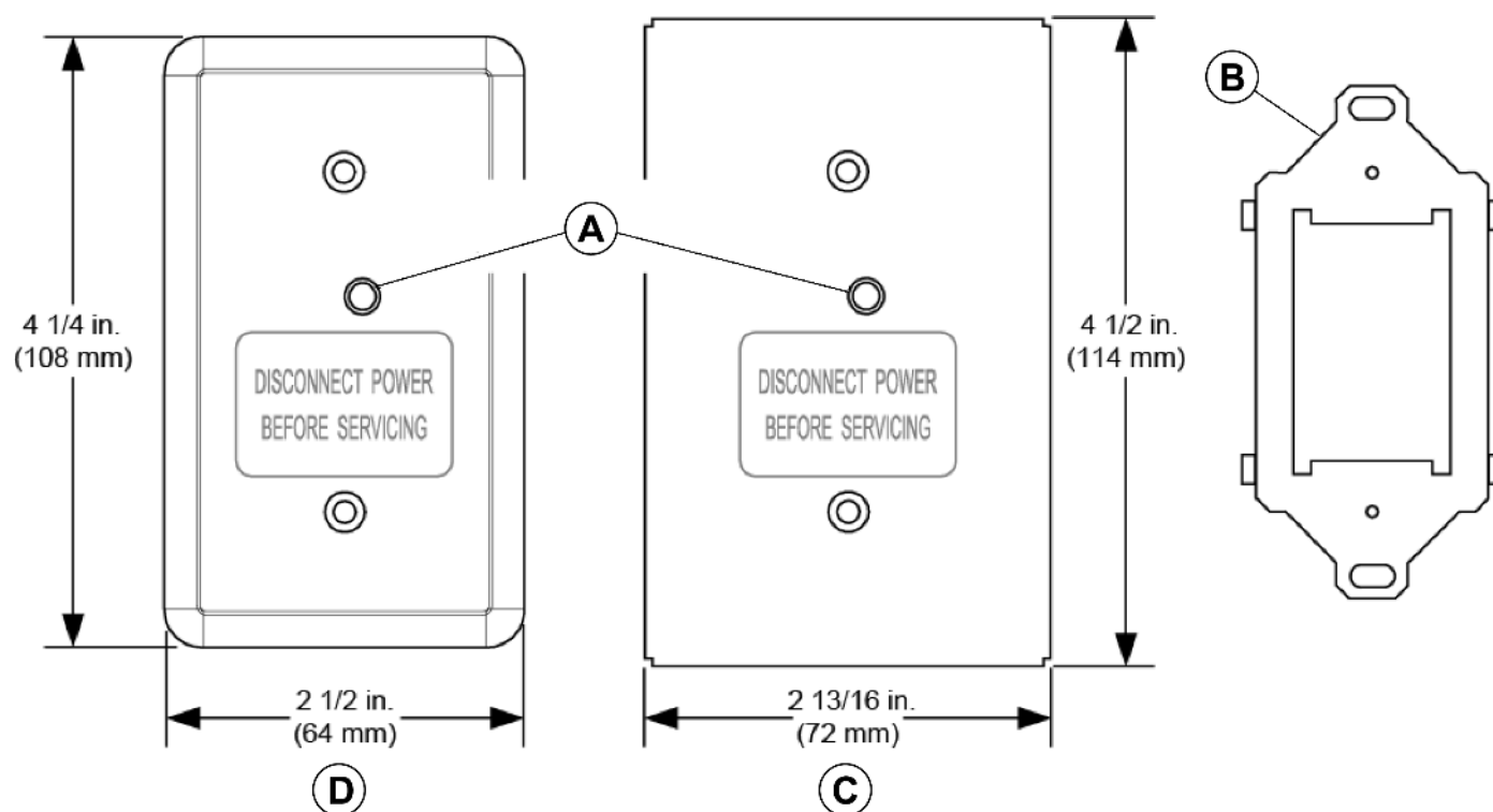
Figure 4: Optional trim plates and mounting bracket for visible LED
